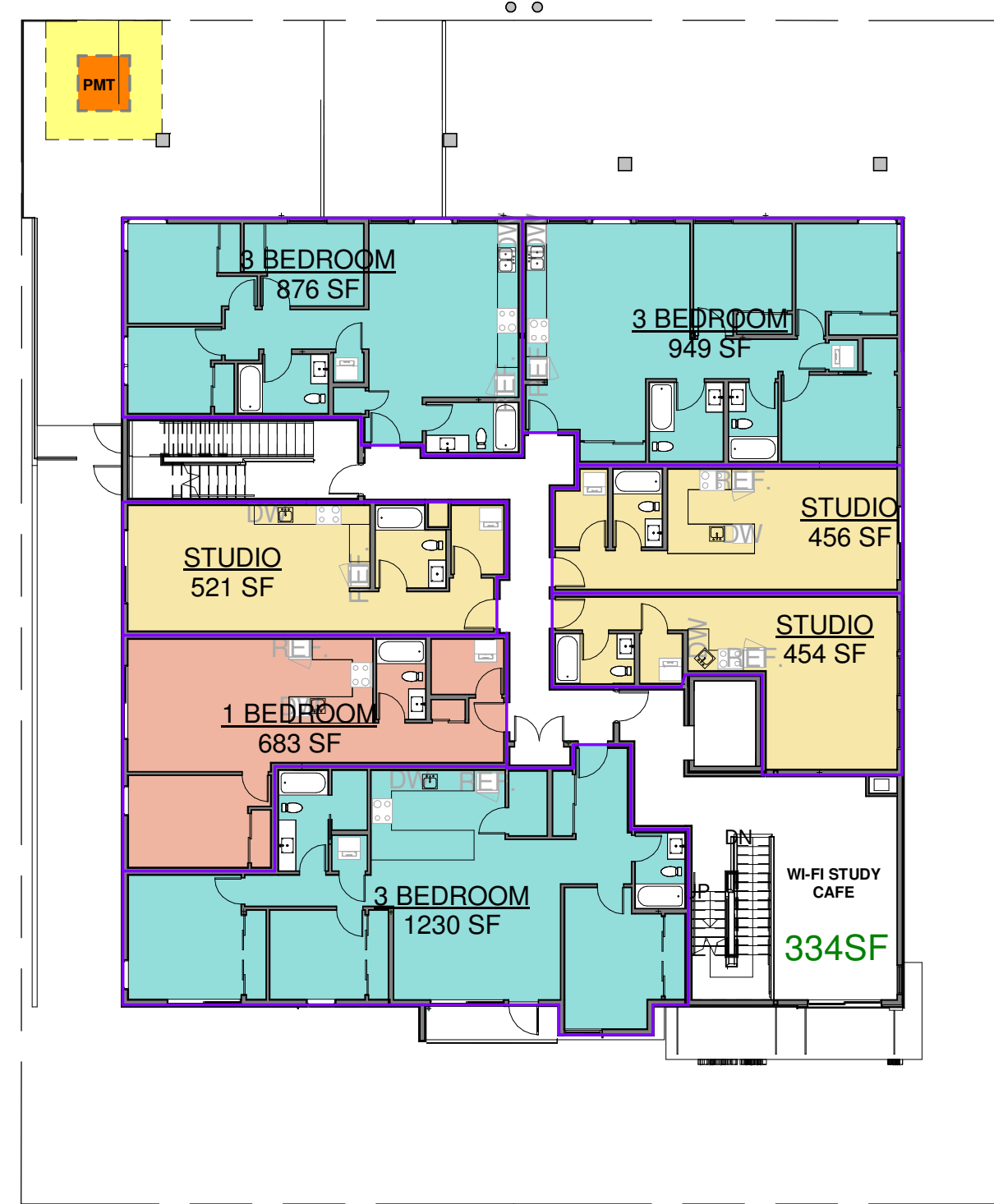
2 L2 1/16" = 1'-0"
